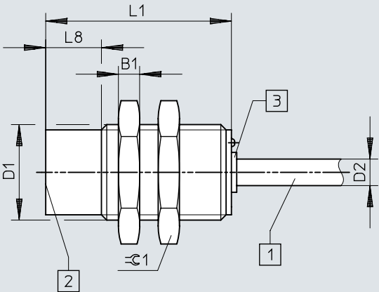
Dimensions – M18, not flush mounted, cable
