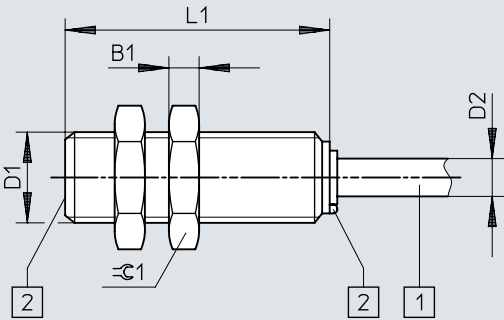
Dimensions – M12, flush mounted, cable
