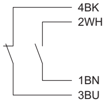
Fig. 3 1 NO + 1 NC (without LED)
